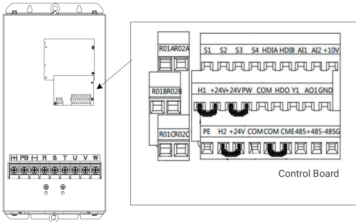
Figure 3 Control Wiring
